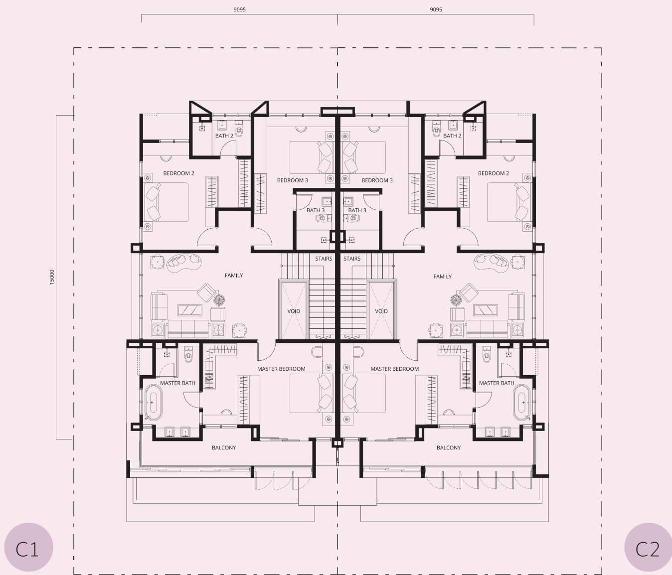
First Floor
